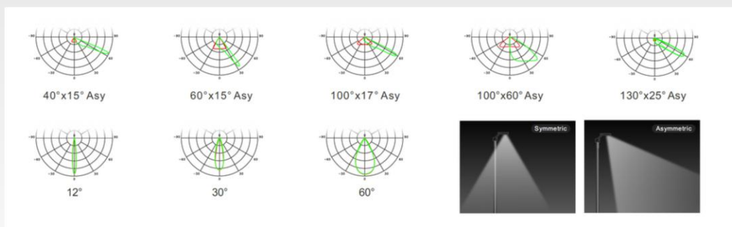
Luminous intensity distribution diagram
