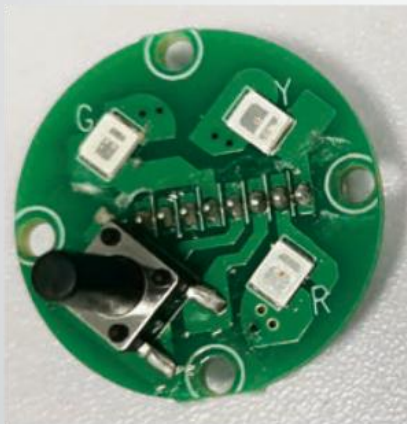
Image: Indicator light LED and Tact Switch
